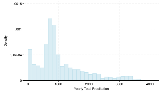
(b) Precipitation
