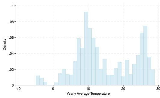
(a) Temperature
